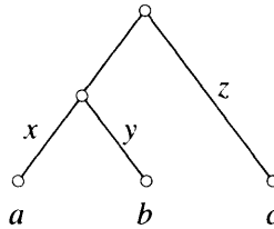
Figure 4.10 Observation for branch lengths.
