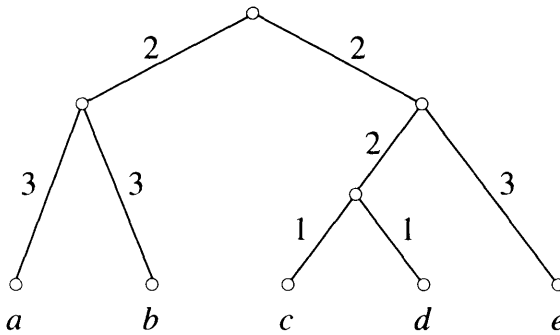
Figure 4.3 Ultrametric topology.
