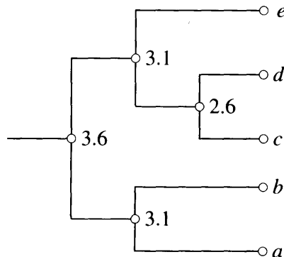
Figure 4.9 Farris transform method.
