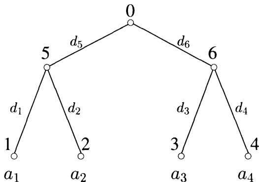
Figure 4.11 Example topology.
