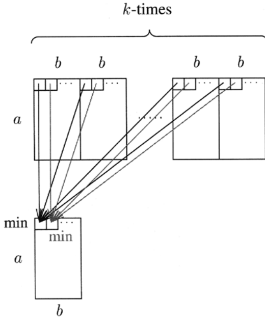
Figure 3.4 Overlay matrix for tandem repeats
