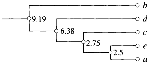
Figure 4.7 UPGMA incorrectly reconstructed topology.
