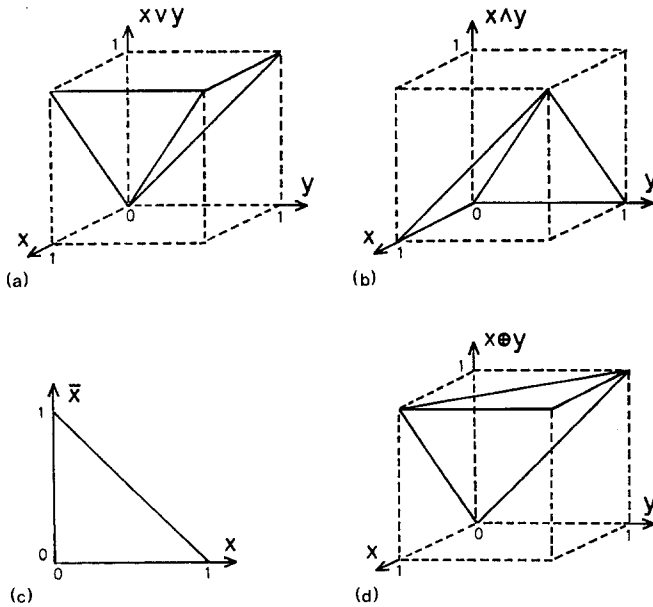
FIG. 1. Illustration of logical operations. (a) Logical sum x \vee y = \max\{x, y\} . (b) Logical product x \wedge y = \min\{x, y\} . (c) Negation \bar{x} = 1 - x . (d) Sum x \oplus y = 1 \wedge (x + y) .
