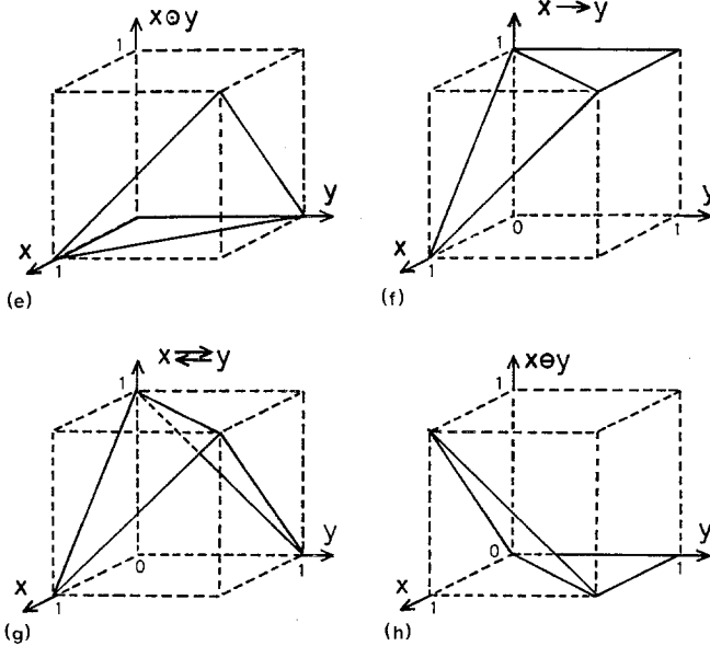
FIG. 1—Continued. (e) Product x \odot y = 0 \vee (x + y - 1) . (f) Implication x \rightarrow y = 1 \wedge (1 - x + y) . (g) Equivalence x \rightleftarrows y = (1 - x + y) \wedge (1 - y + x) . (h) Difference x \ominus y = 0 \vee (x - y) .
