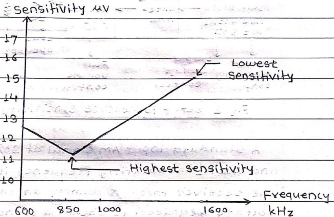
Fig. 1: Sensitivity curve
