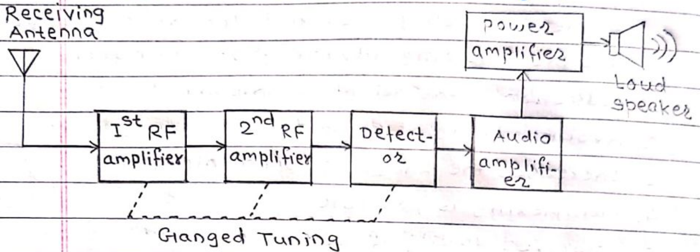
Fig 1 The TRF Receiver
