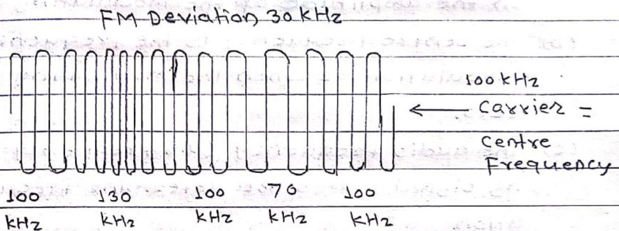
Fig 2 FM signal
