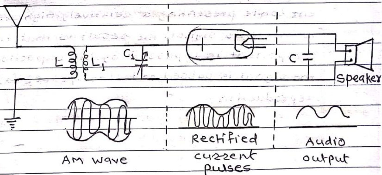
Fig. 1 AM diode Detector
